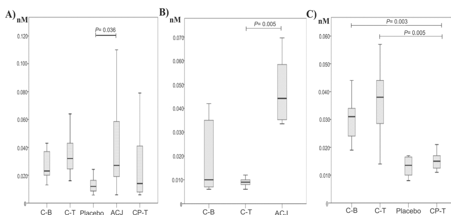
Fig. 3 Box plots with quartiles (upper values 75%, median 50%, and lower values 25%) of the concentrations of DNA metabolites in plasma throughout the study (nM). Friedman's ANOVA and post hoc analysis with Wilcoxon signed-rank tests (with a Bonferroni correction) were conducted. (A) cGMP ( P < 0.05 , only the ACJ and placebo stages were compared), (B) 8-NO 2 -Gou ( P < 0.016 ), and (C) 8-OH-Gua ( P < 0.005 ). Abbreviations: C-B: control baseline, C-T: control training, ACJ: aronia–citrus juice, CP-T: control post-treatment.
