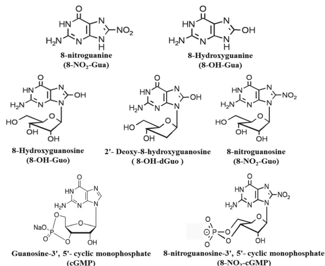
Fig. 2 Chemical structures of the seven DNA oxidation catabolites analyzed in this study.
