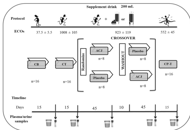
Fig. 1 Study design. This was a randomized, double-blind, and placebo-controlled crossover study. Sixteen athletes, randomly divided into two groups, were assigned to supplementation with either 200 mL of ACJ or 200 mL of placebo. After 45 days of supplementation and a 10-day washout period, the beverages were swapped during the same period (45 days). Three controls were used: baseline control (C-B), control-training (C-T), and control post-training (CP-T), with a duration of 15 days. The samples (urine/blood) were collected at rest and under fasting conditions, on the last day of each stage. The training load was quantified by the Objective Load Scale (ECOs).
